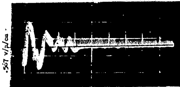
Fig. 3.74 Broadband pulse Shot No. 6 1000 km from ground zero
